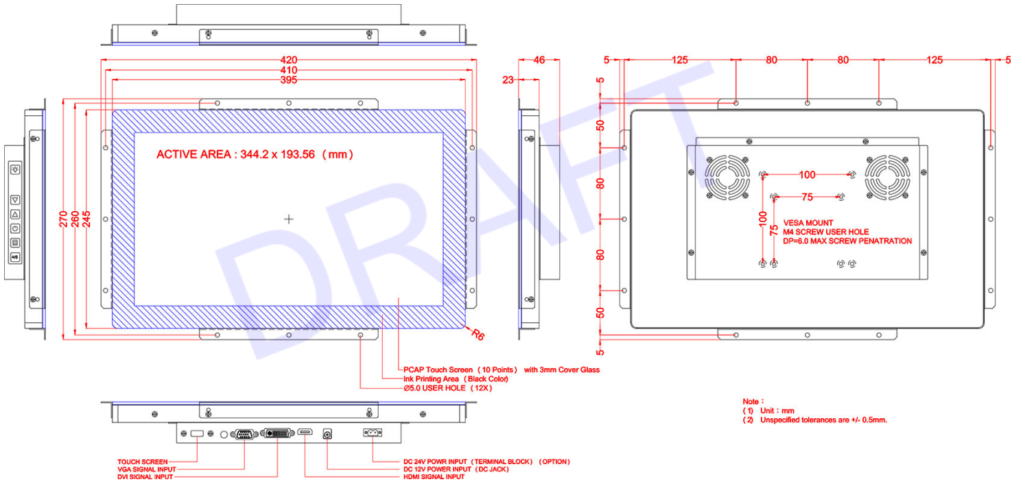
Drawing No.: YOPW1560HB-TPCT-24V-02032023-V2
