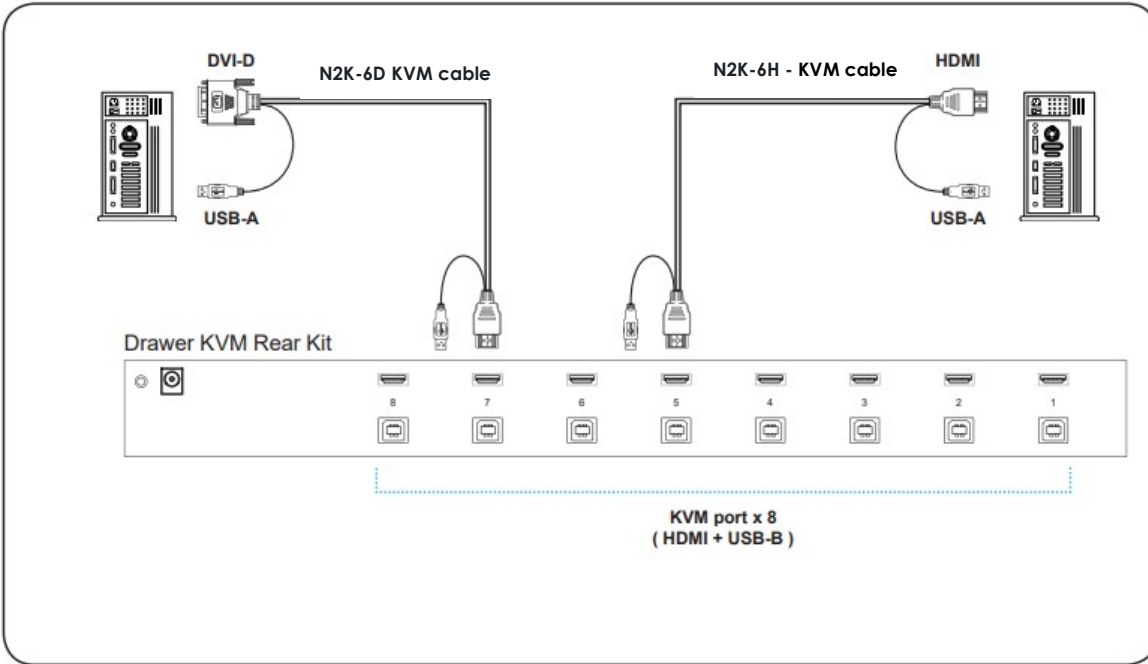
N2K-6D - 6 feet DVI-D KVM cable ( Server end : DVI-D + USB-A ) ( KVM port : HDMI + USB-B )
