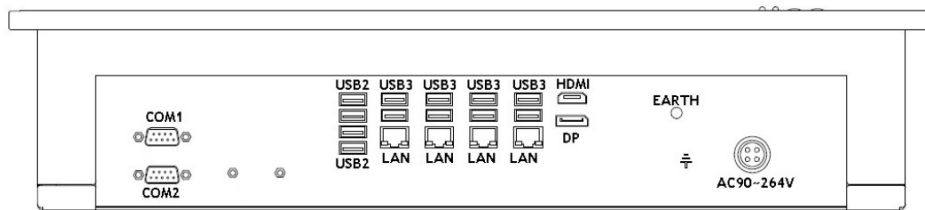
I/O Ports
