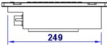
Side View 1
