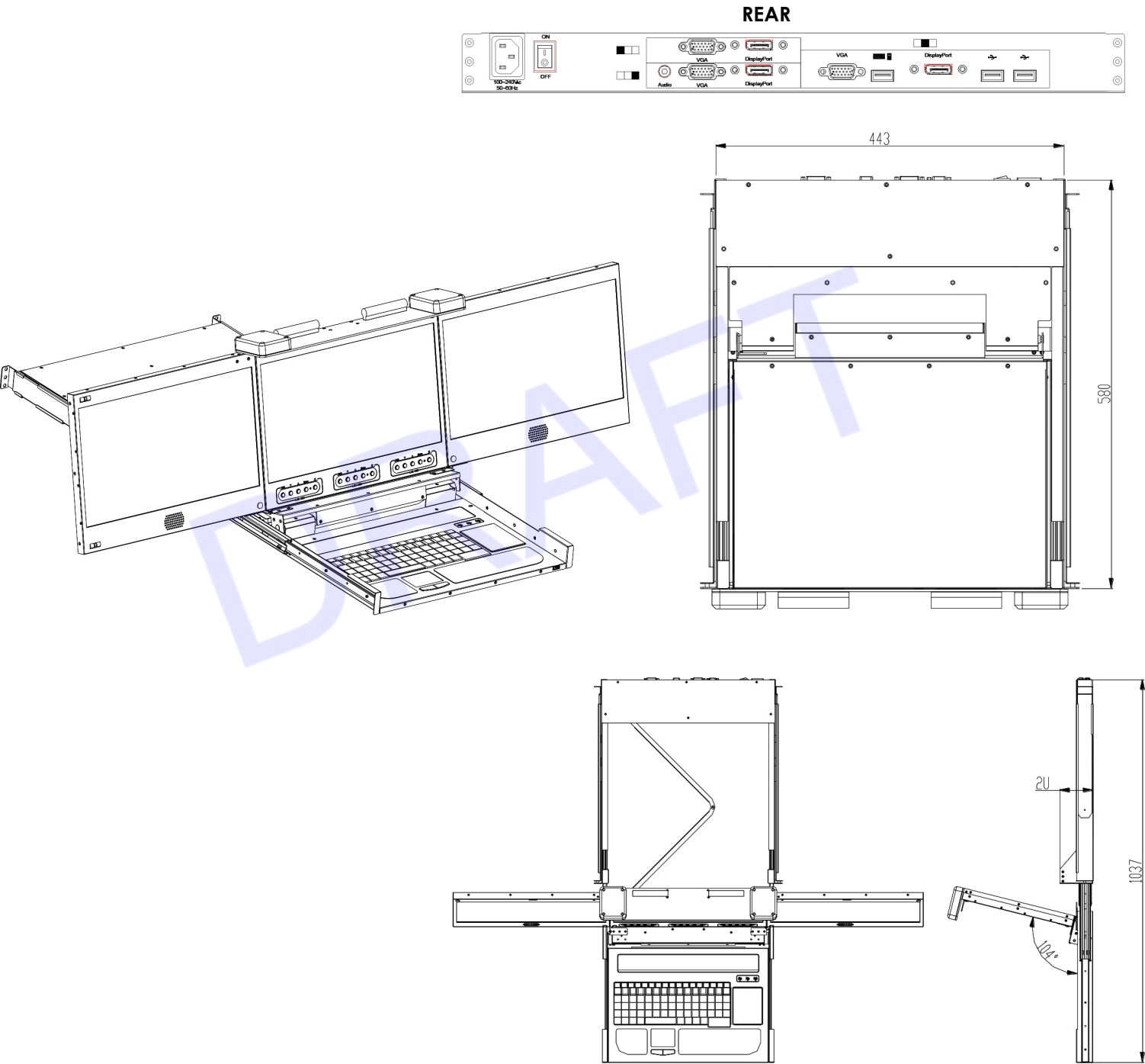
Drawing no.: ASK3D1730-DPV-11012022-V1
